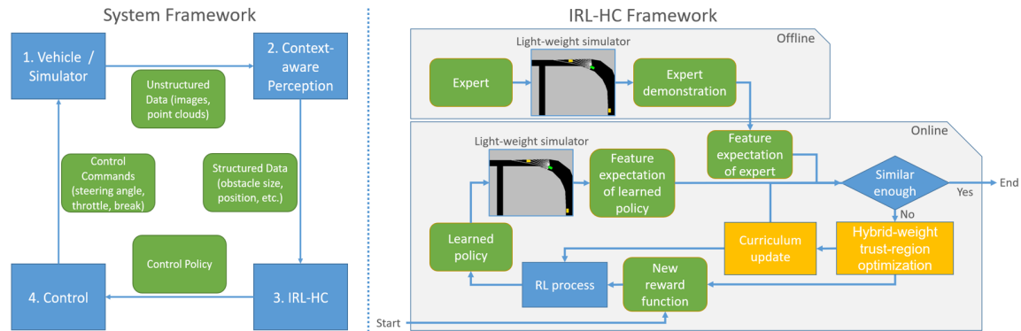
Fig. 1. System Pipeline (LEFT) . At each time step, the vehicle/simulator generates unstructured data such as images and point clouds. These data are processed by the perception module to produce structured data, which are then used by the IRL-HC module to learn a control policy for autonomous driving. IRL-HC training process (RIGHT) . We compute the expert trajectories offline. Next we use hybrid-weight trust-region optimization to obtain a new reward function, which is then used to compute the feature expectation of a learned policy online. The curriculum difficulty will also be updated progressively, according to the trust-region updating rules that assess the learned task difficulty.
